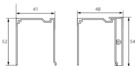
Takmontering.
